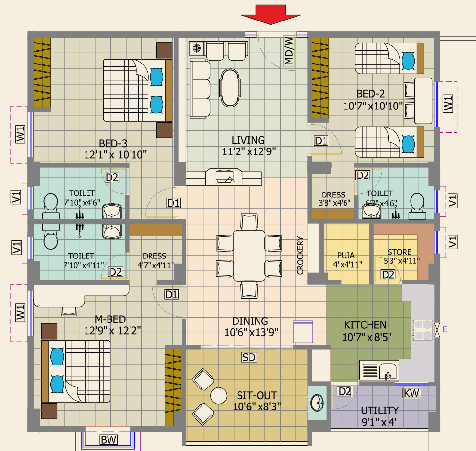
3 BHK DELUXE | SOUTH FACING | 1487 SFT.
